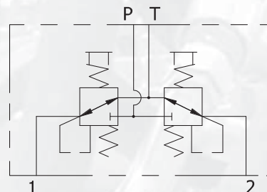
HYDRAULIC SCHEMATIC
