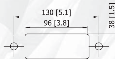
INSTALLATION PATTERN
